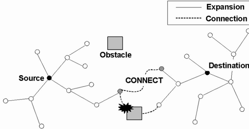
FIGURE 4.8 : Probabilistic Roadmap.
