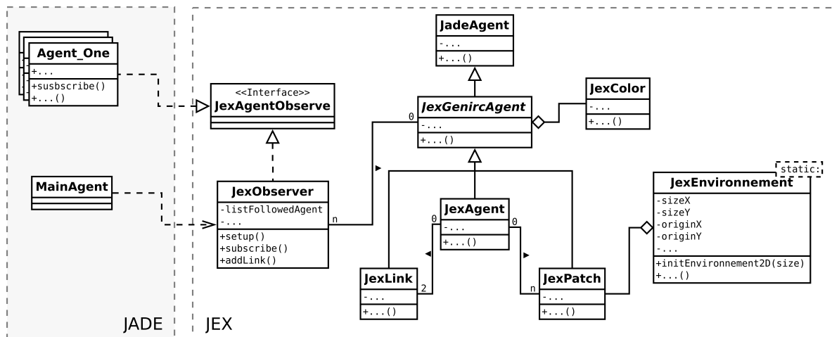
FIGURE 5.6 : Architecture JEX : diagramme UML.
