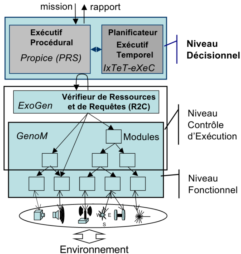
FIGURE 2.6 : Architecture LAAS.
